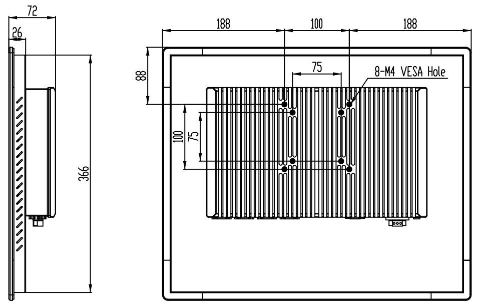
CUT OUT DIMENSION (454mmx368mm) UNIT:mm
